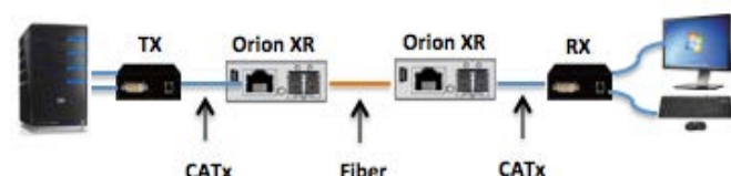
Fiber long distance extension. CATx to fiber
