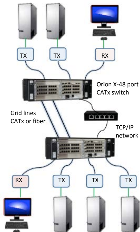
Structure of a matrix grid network
