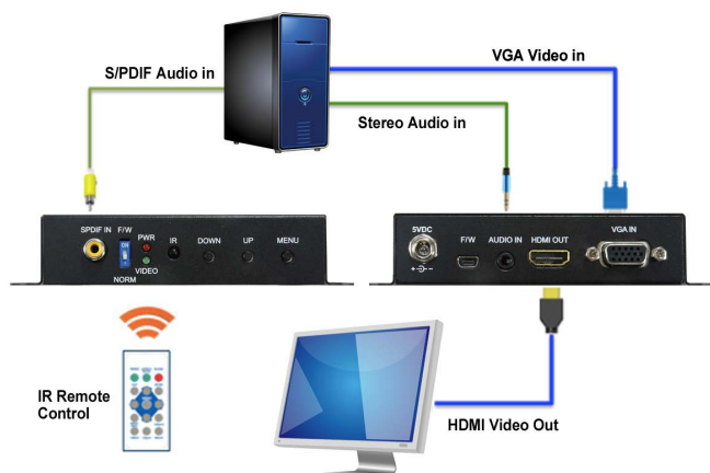
Translator VGA to HDMI connection diagram
